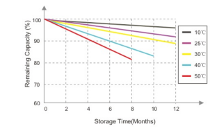
SELF-DISCHARGE CHARACTERISTICS
