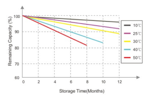
SELF-DISCHARGE CHARACTERISTICS
