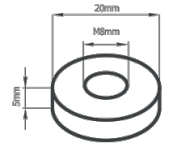
TERMINAL DIMENSION
