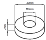
TERMINAL DIMENSION
