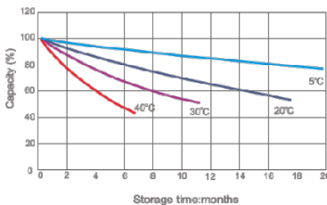
SELF DISCHARGE CHARACTERISTICS
