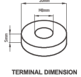
TERMINAL DIMENSION
